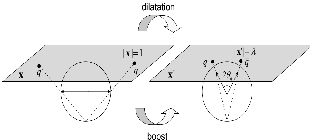
Figure 5. Boosting the q\bar{q} pair in e^+e^- annihilation corresponds to changing the size of the dipole in high energy scattering.
